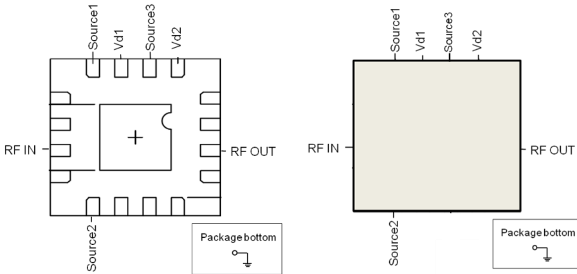
VRFA0026-QFN Top View
